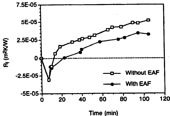
Fig. 8. Fouling resistances vs time for two different cases: without and with electronic anti-fouling (EAF) device. Concentration of test solution = 7.5 \text{ mol m}^{-3} ; cold water flow velocity = 0.65 \text{ m s}^{-1} ; hot water flow velocity = 2.23 \text{ m s}^{-1} ; hot water inlet temperature = 355\text{K} .
